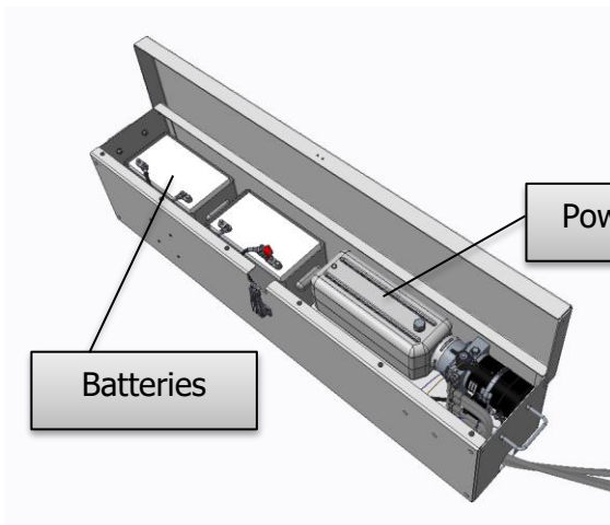
Figure 2 - Hydraulic Power Unit (HPU300 shown)
