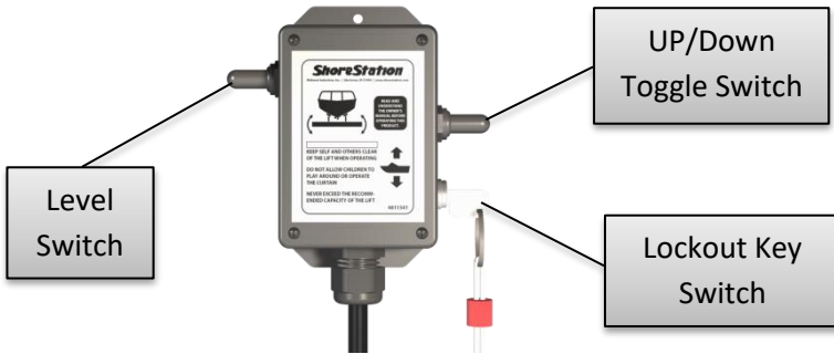
Figure 4 - Wired Dock Switch
