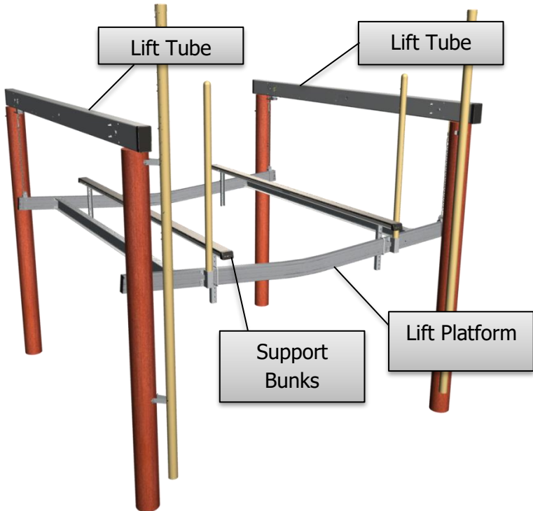
Figure 1 – ShoreStation Boat Lift Components
