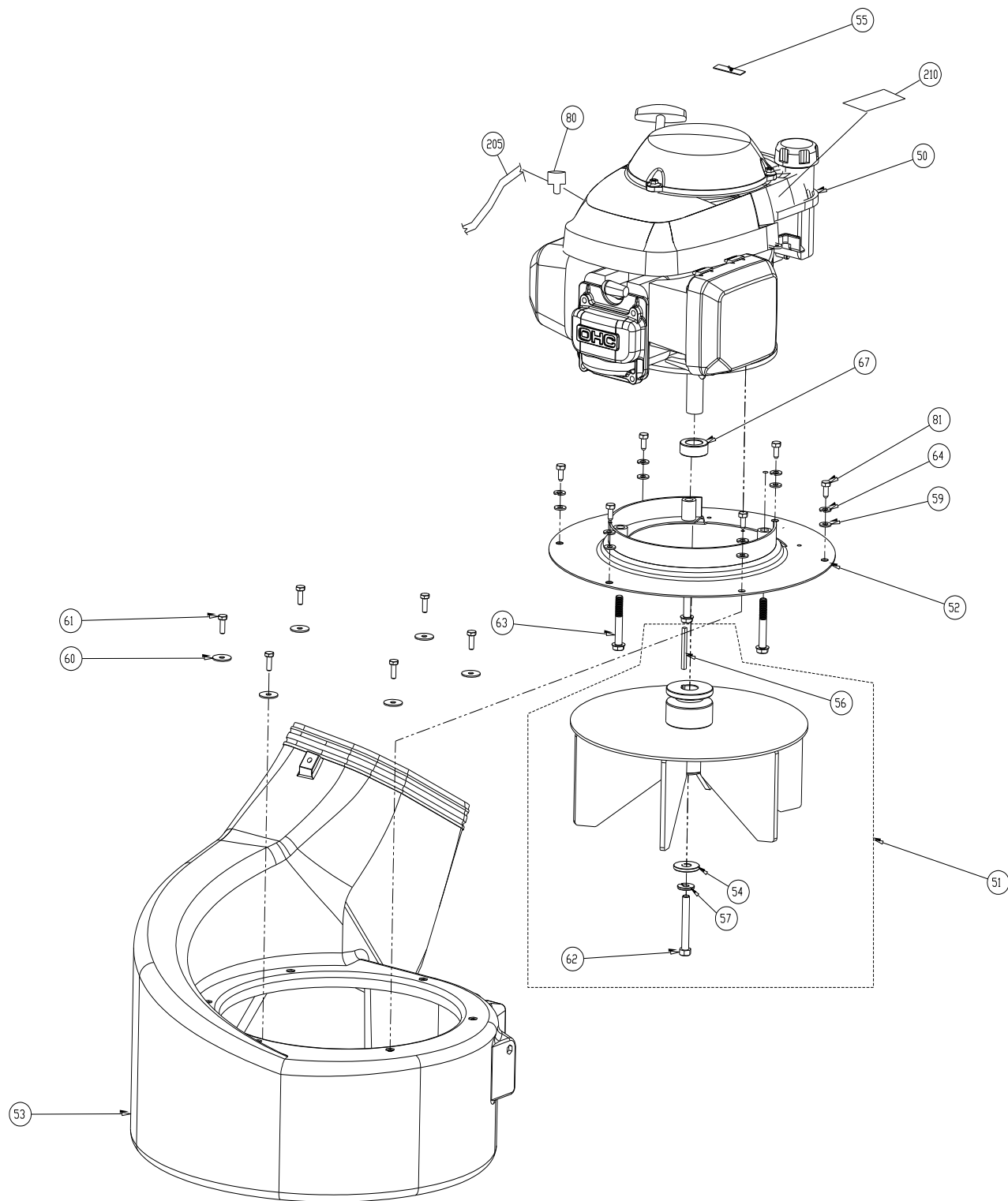
Engine Assembly
