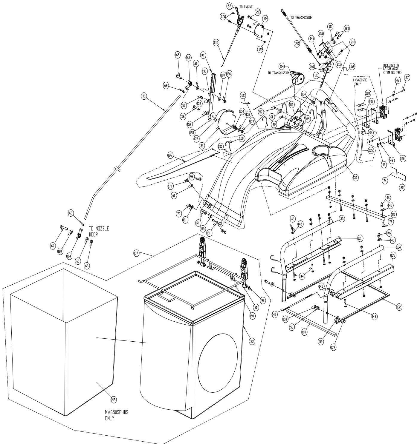
Hood Assembly
